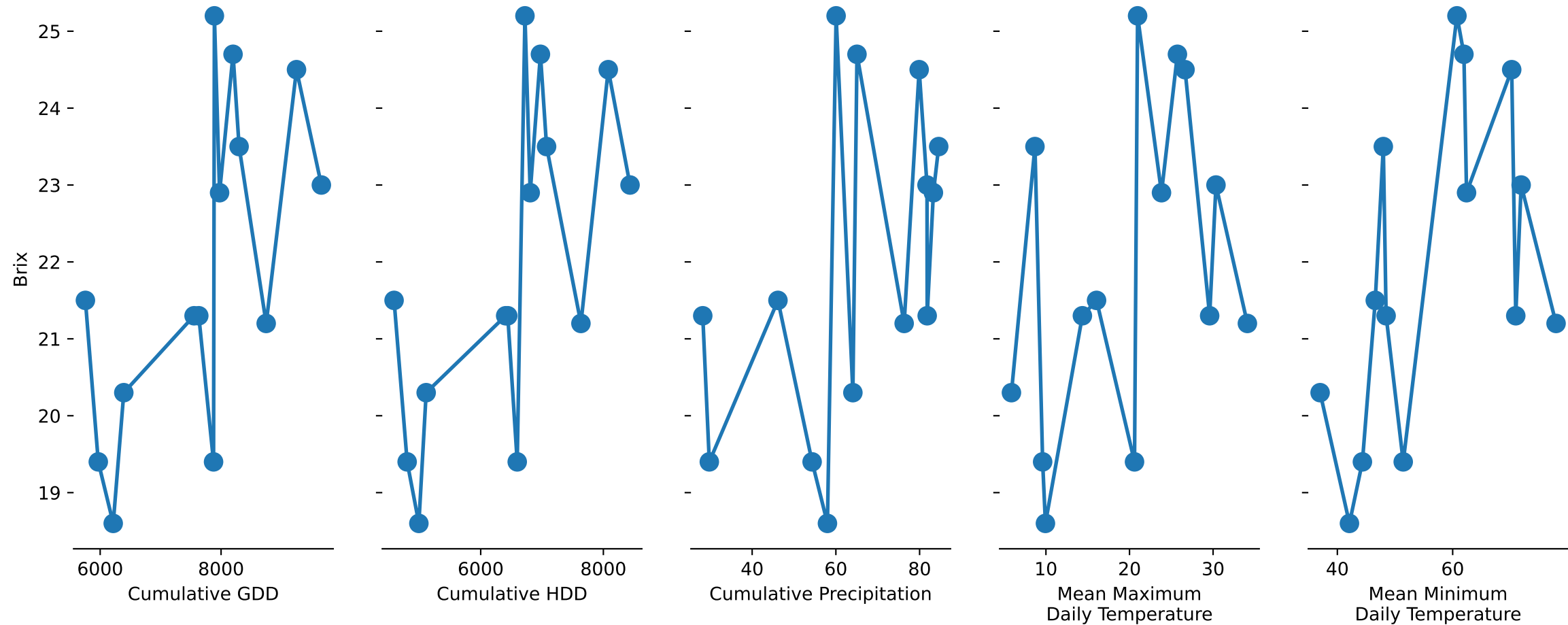
Climate impacts on Brix for Marquette, 2019
